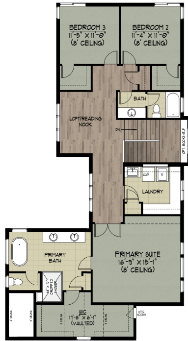
UPPER FLOOR PLAN
