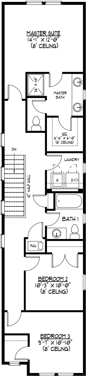
UPPER FLOOR PLAN
