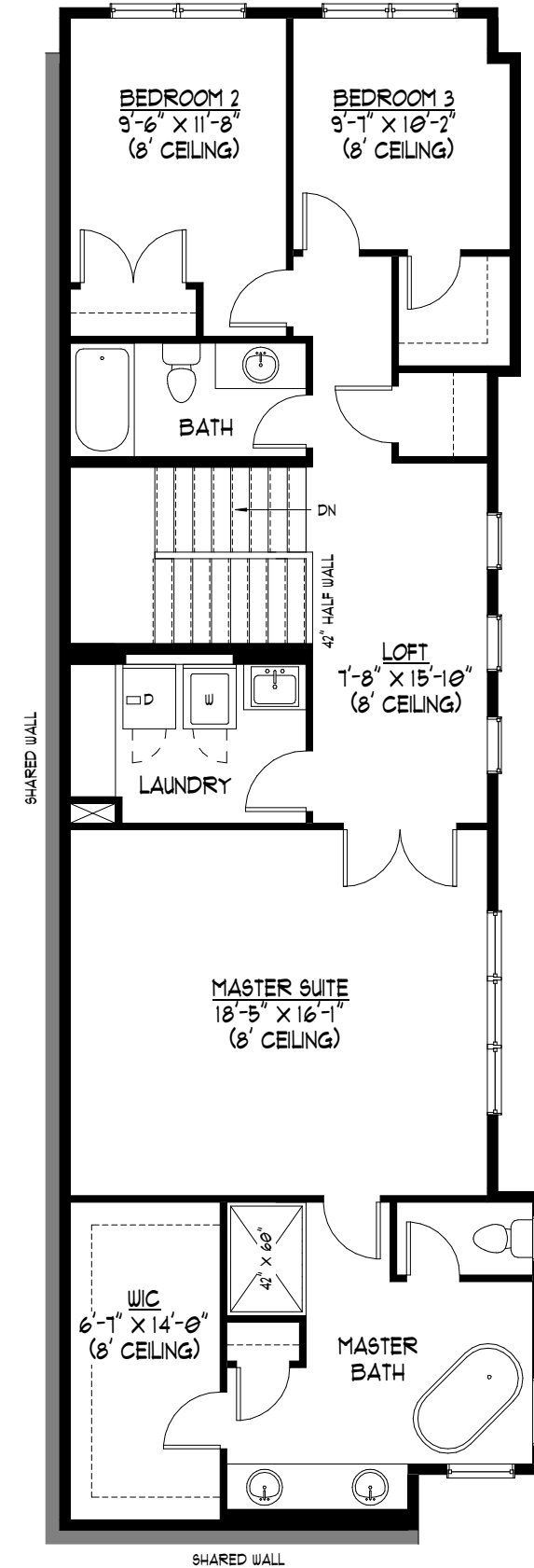
UPPER FLOOR PLAN
