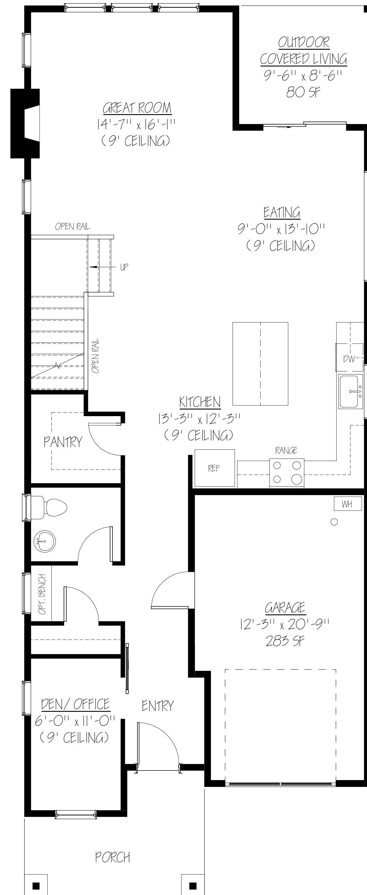
MAIN FLOOR PLAN
