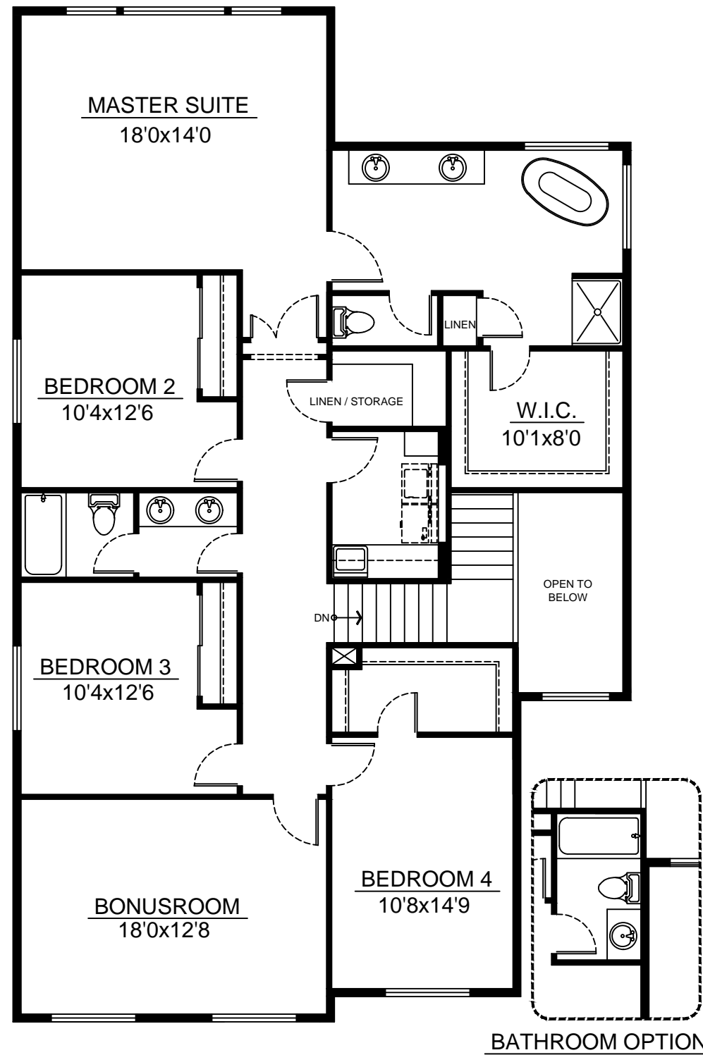
UPPER FLOOR PLAN 1,766 S.F.
