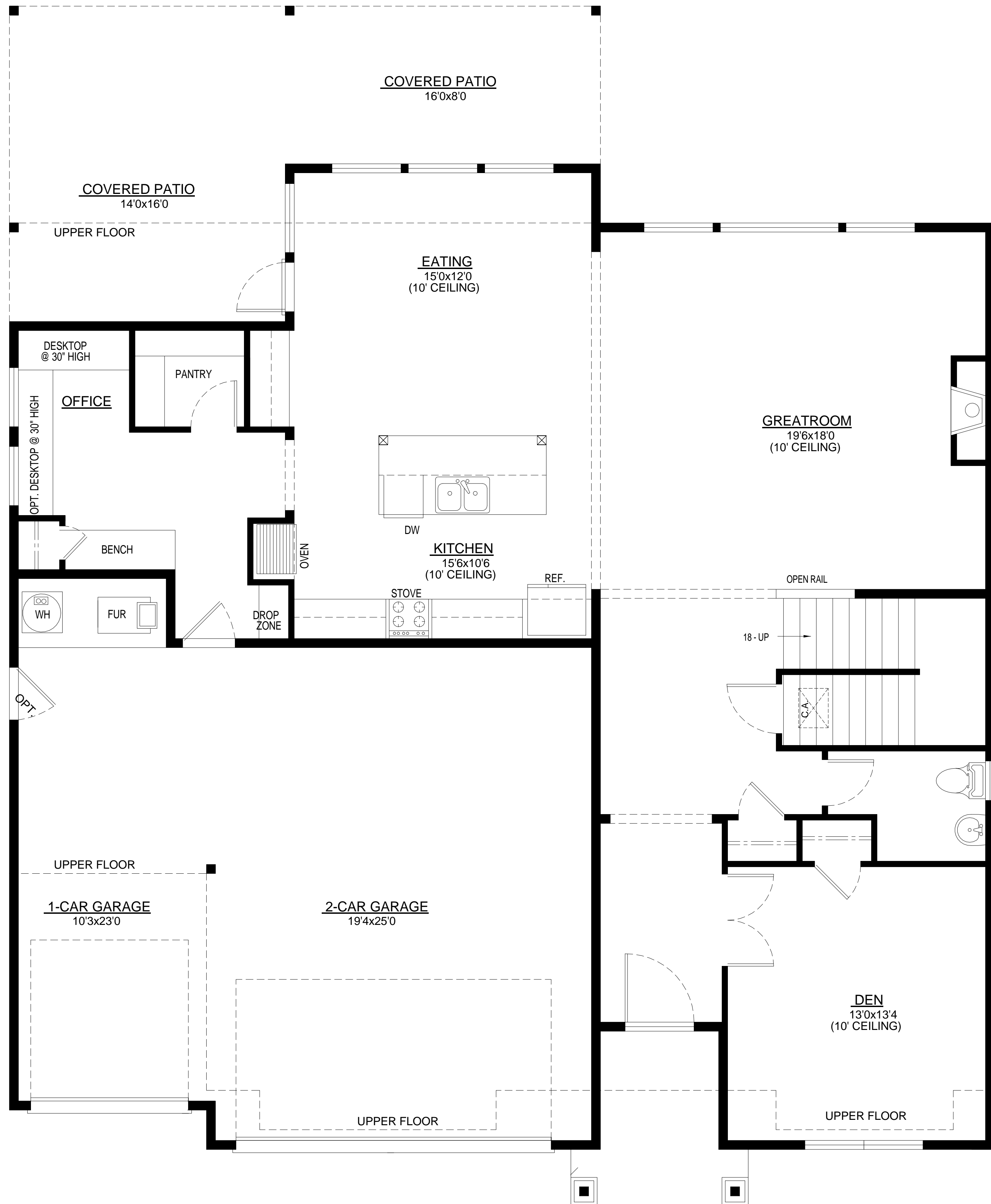
MAIN FLOOR PLAN
