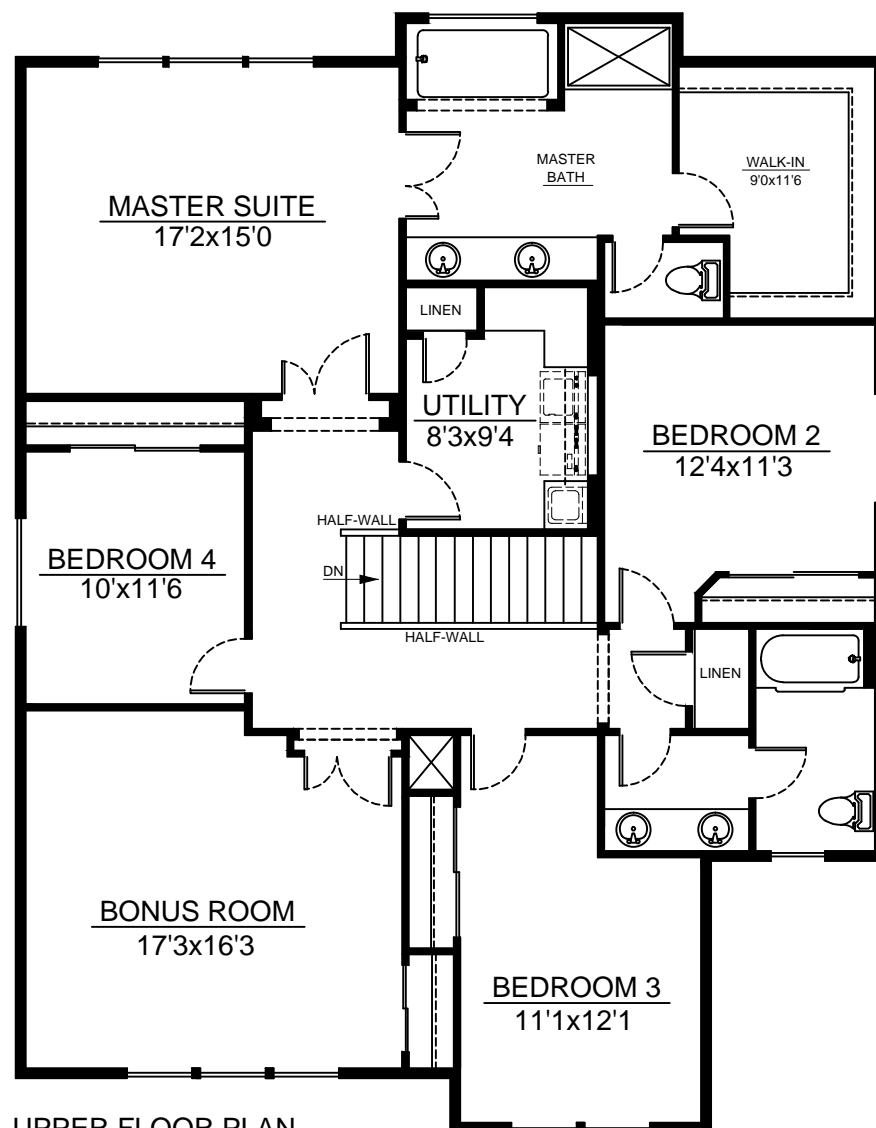
UPPER FLOOR PLAN 1,810 SQ.FT.
