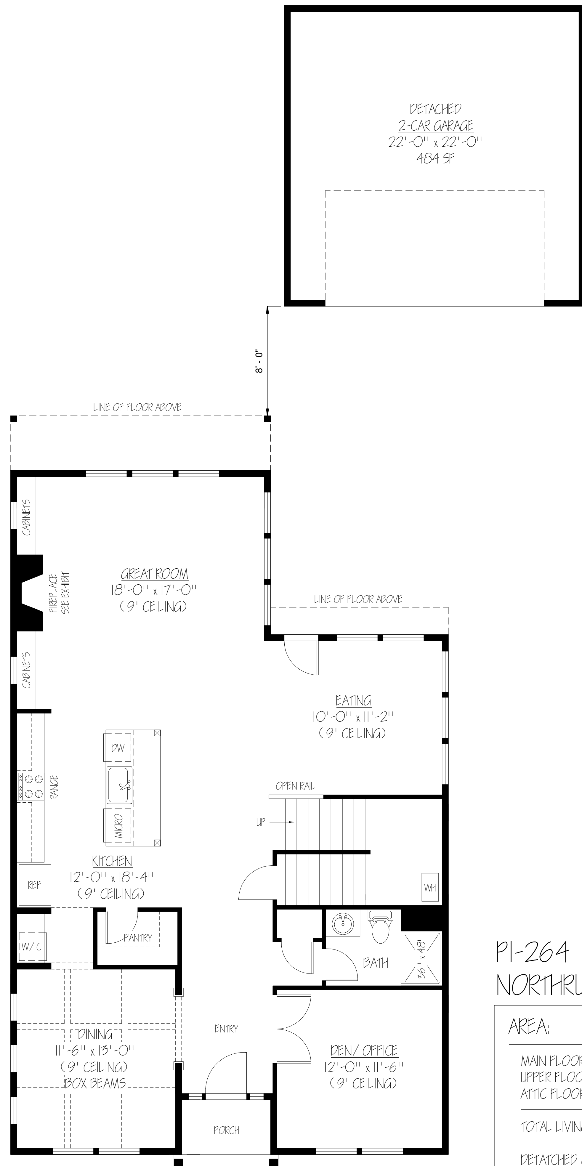
MAIN FLOOR PLAN
