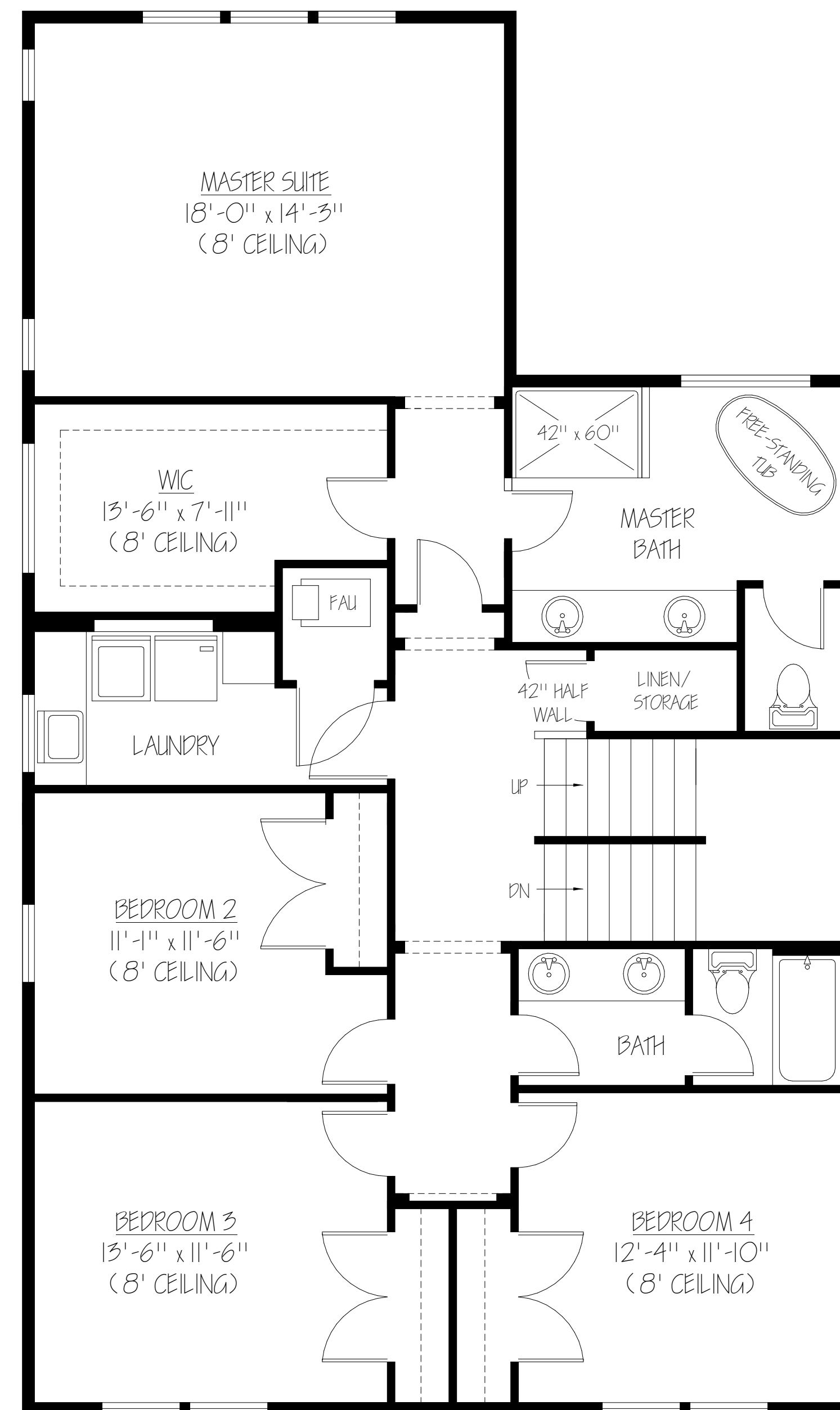
UPPER FLOOR PLAN
