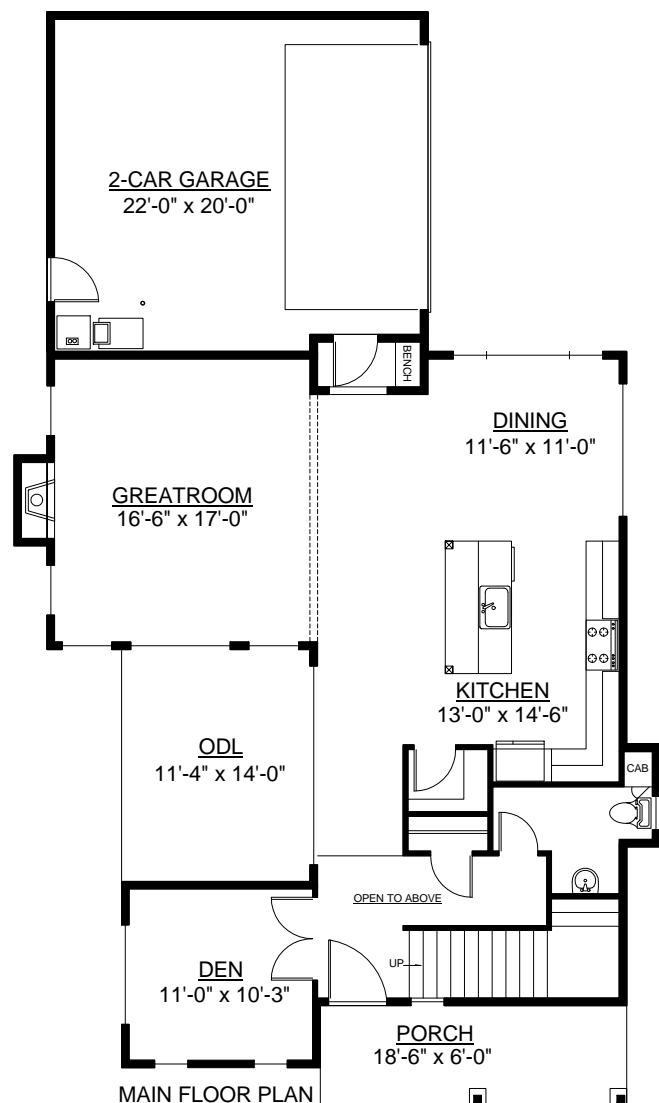
MAIN FLOOR PLAN 1,193 SQ.FT.
